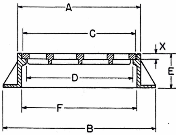
Flat Grate
