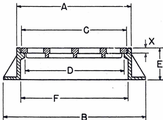
Flat Grate
