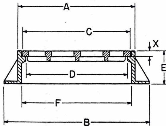
Flat Grate
