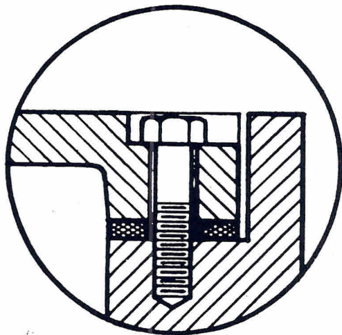
Bolting Detail
